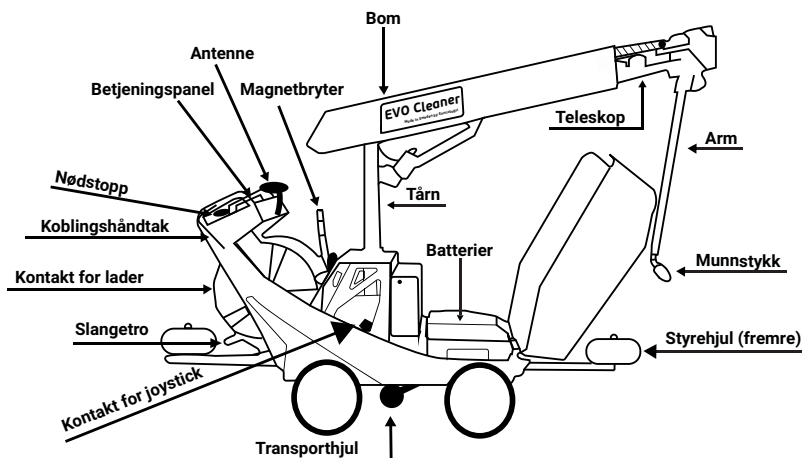
Figur 2, robotens deler
